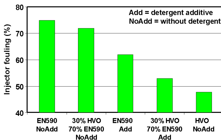
Figure 22. Injector fouling tests a) with DW10 engine [Neste Engine Laboratory tests], and b) with XUD engine where lower values are better [Neste Engine Laboratory tests]. The fuels used for the tests included EN590 diesel fuel and HVO (Neste Renewable Diesel).
