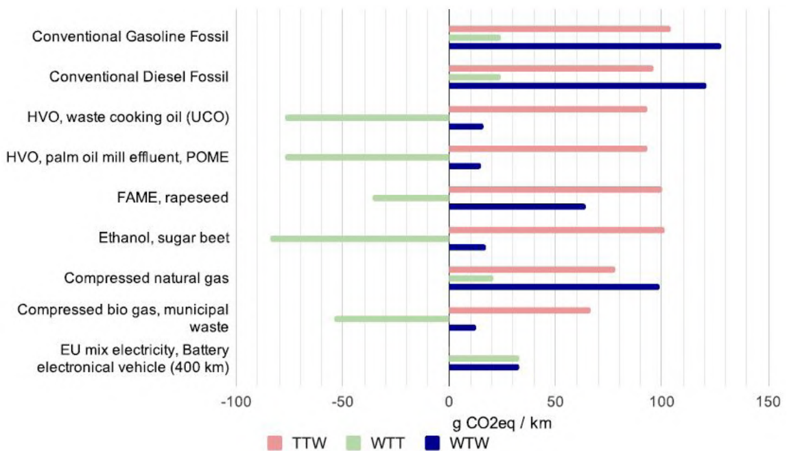
Figure 11. Well-To-Wheels greenhouse gas emissions of a typical midsize class car, 2025+ as emissions/km. WTT means Well-To-Tank (emissions from fuel production chain) and TTTW means Tank-To-Wheels (tailpipe emissions). In the JEC WTW methodology, carbon sequestration is taken into account in the WTT part. WTW is the sum of WTT and TTTW. [Prussi et al. 2020]
