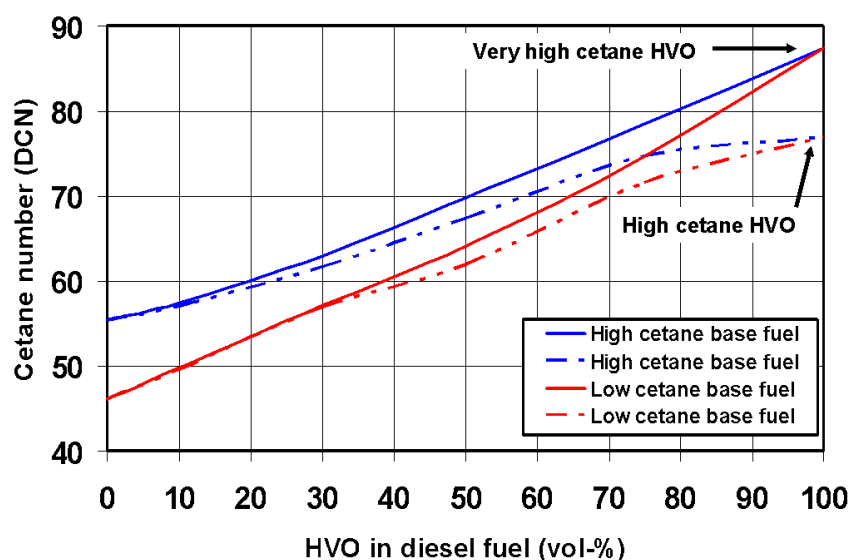
Figure 6. Cetane number of two different Neste renewable fuels (HVO: high and very high cetane) blended with two different diesel fuels (low and high cetane).
